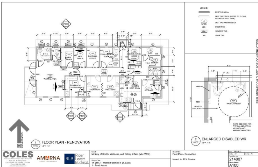
Figure 3 & 4 Site Plan and Floor Plan for the Fond Assau Wellness Centre Rehabilitation
