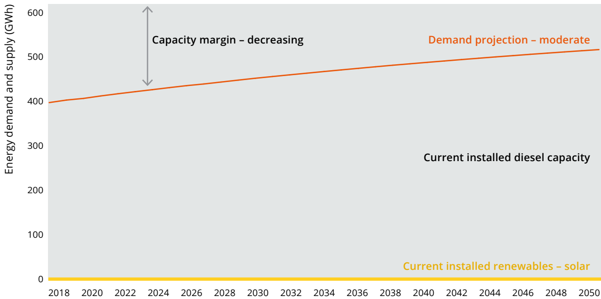
Figure 7: Future needs under a moderate demand growth scenario, electricity sector
